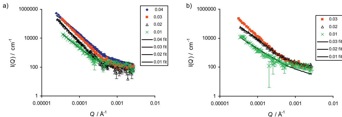
Fig. 4. Ultra small-angle scattering from flocculated hydrogenous latex, PS3, (a) with Moringa oleifera . Different particle concentrations (mass fraction) are shown with fits, (b) flocculated PS3 with Moringa stenopetala protein.
